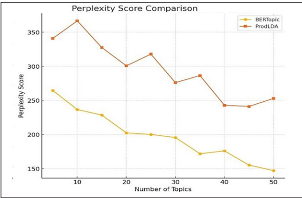
Figure 10. Perplexity score comparison between BERTopic and ProdLDA
